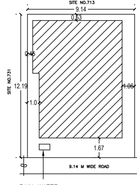
SITE PLAN
