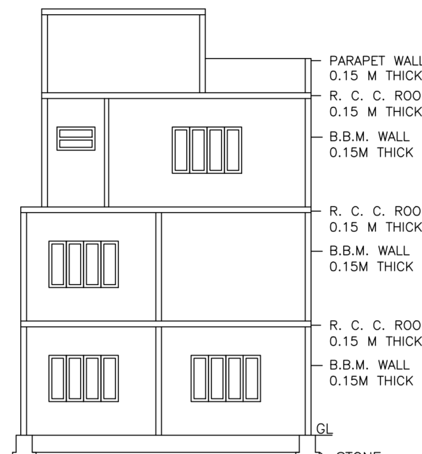
SECTION AA
