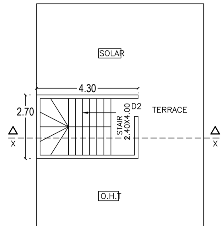
PROPOSED TERRACE FLOOR
